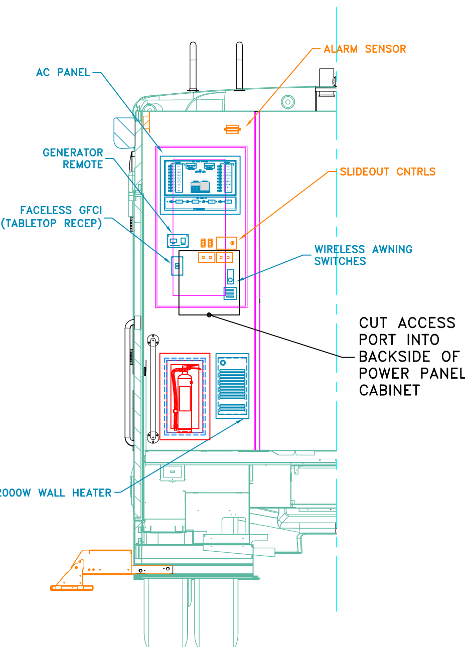
SECTION F-F
